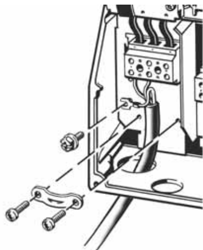
Fig. 33 Mains connection
